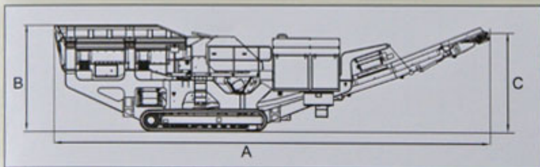
J-1175 Jaw Crusher in Working Position
