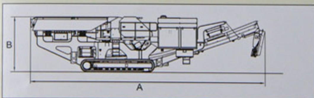
J-1175 Jaw Crusher in Transport Position
